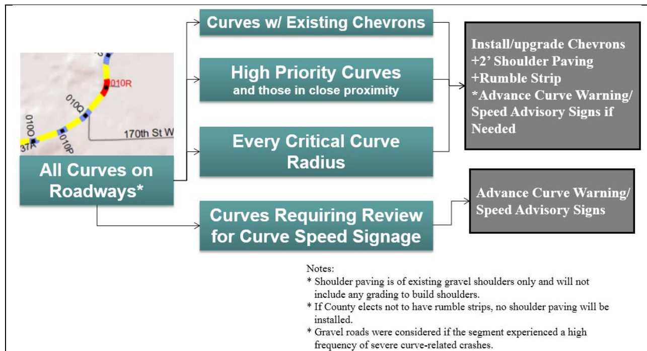
FIGURE 4-2 High-Priority Rural Curve Project Decision Tree
